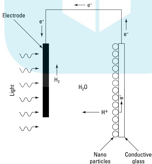
Figure 9-3: A photoelectrochemical cell.
